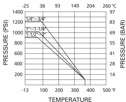
PRESSURE-TEMPERATURE RATING
